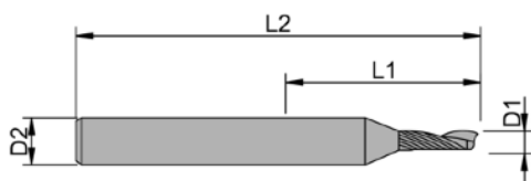
Reduced diameter
